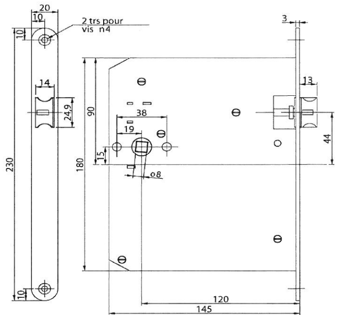
VERSION BEC DE CANE A CONDAMNATION NB01221600
