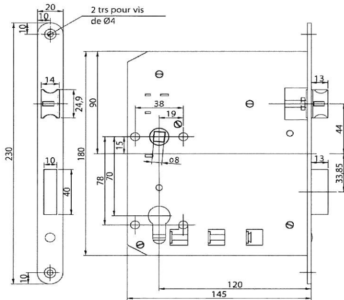
VERSION PENE DORMANT 1/2 TOUR NB91201600
