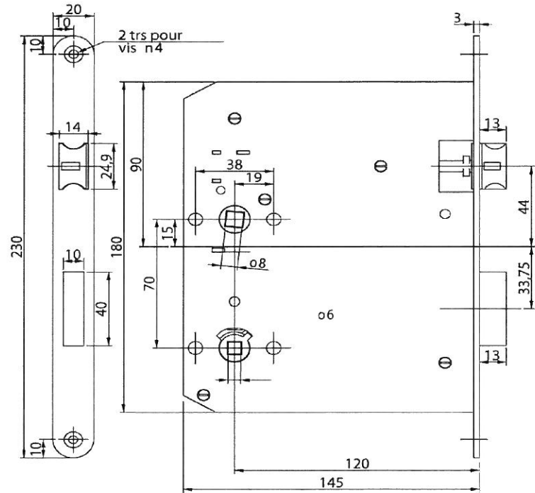
VERSION BEC DE CANE A CONDAMNATION NB01221600
